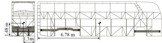
Figure 2. Location of the center of gravity of the bus structure
