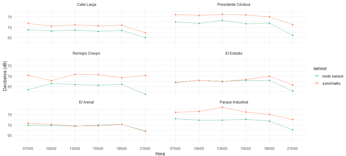
Figure 6. Comparison of the emissions made with sensor and sound level meter.
