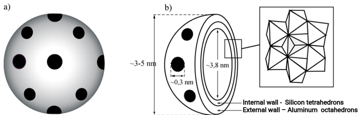
Figure 2. a) External morphology of an allophane nanoparticle. b) Detail of the internal structure.
