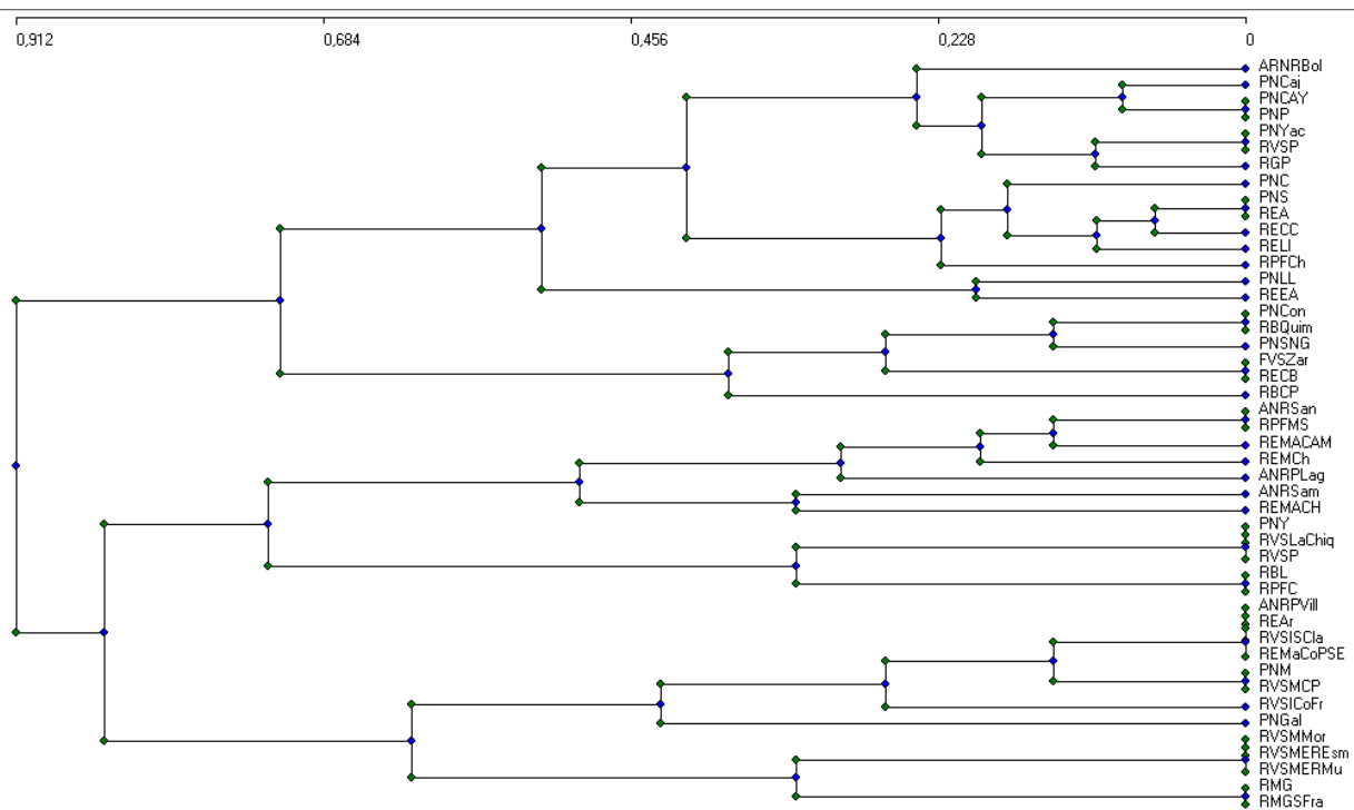
Figure 4. Cladogram of the Protected Areas of the Natural Patrimony Areas of the Ecuadorian state in function of the presence or absence of different ecosystems in them (Appendix 2).
